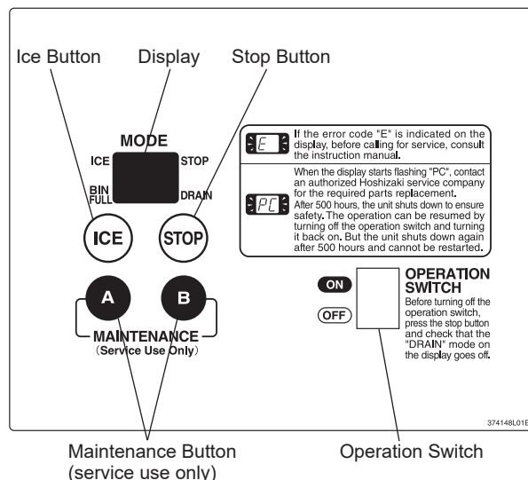
Operation Panel
